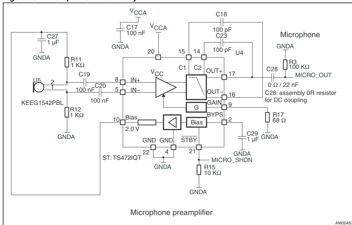
Figure 18. Microphone functionality
