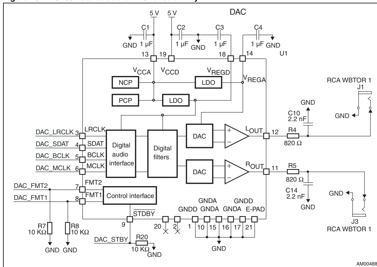
Figure 19. TS4657 stereo audio DAC functionality
