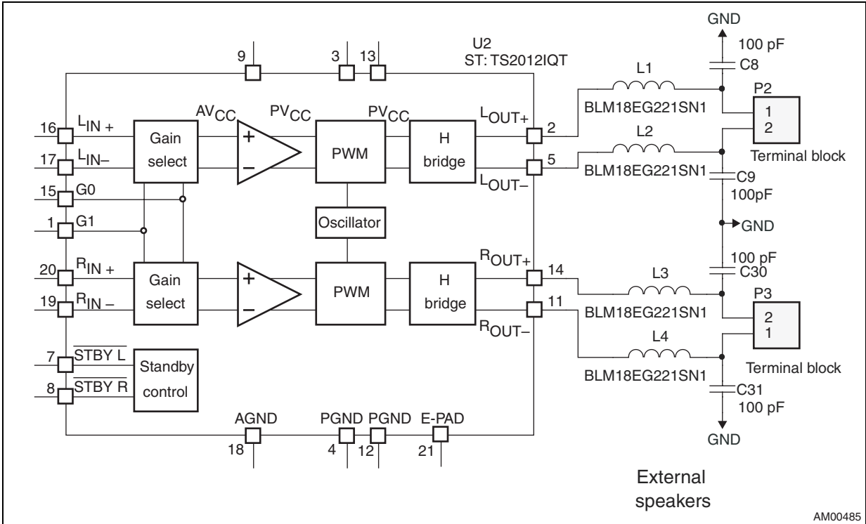
Figure 16. TS2012 stereo output terminal connectors P2, P3
